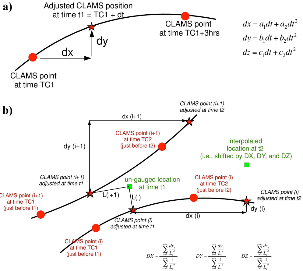
Figure 2: Data processing: the spatio-temporal interpolation technique. a) ADJUSTT: a_1, a_2, b_1, b_2, c_1, c_2 are pre-calculated at every CLaMS position using least squares and added as new attributes to CLaMS data sets. Three position (the current position and the subsequent two positions) are used in the least squares to pre-determine the coefficients at each clams position on the regular 3-hours CLaMS scale. b) SPATIOT: n is the number of nearest neighborhood CLaMS points used in the interpolation (recommended n = 5-16 , 9 is used).
