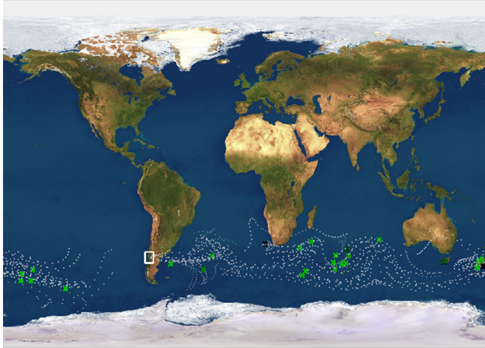
Figure 6: Task 2: Temporal evolution of MIPAS detections for Puyehue-Cordón Caulle eruption (overlaid on CLaMS trajectories).
